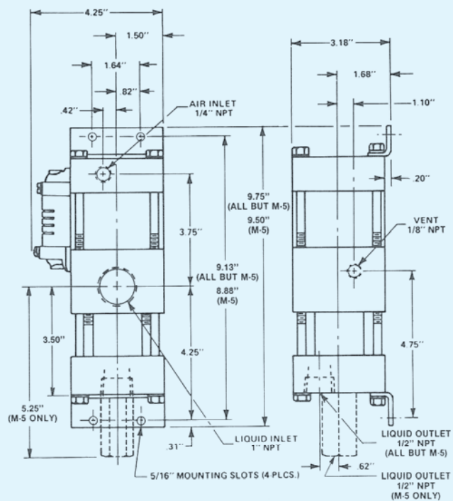
MDSTV-5 & MDTV approx. weight 15 1/2 lbs (7 kg)
