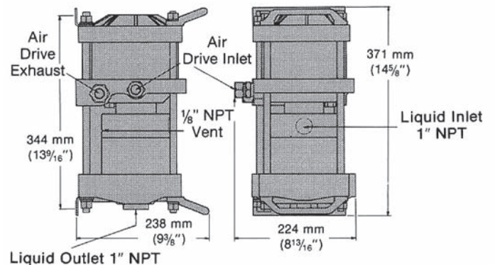
DSTV-1.5 pump; single acting, high output
