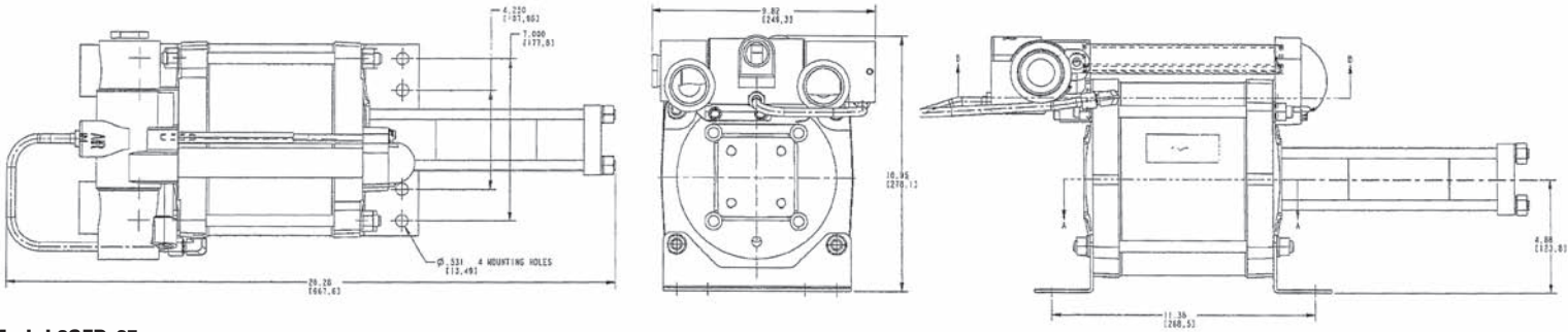
Model 8SFD-65
