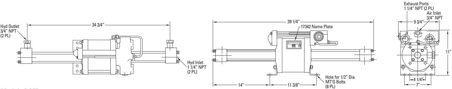
Model 8DSFD-100
