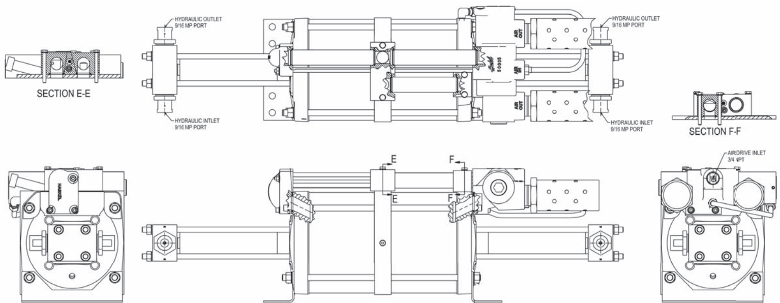
Model 8SFD-224
