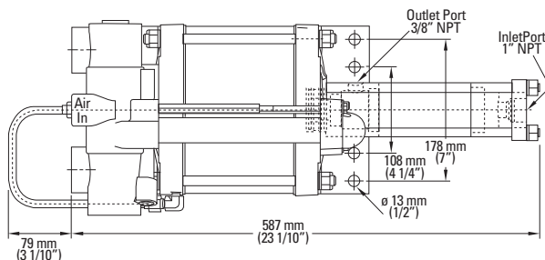
Model 8SFD-40
